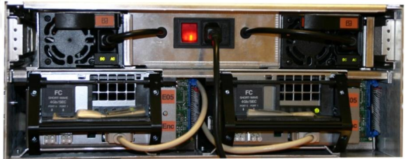
ALL HOT SWAP COMPONENTS ACCESSIBLE FROM THE REAR
